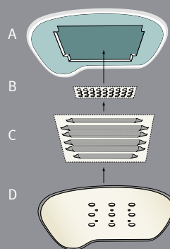
A Cold-foam cushion. B Spiral springs. C Spring system. D Base plate.
